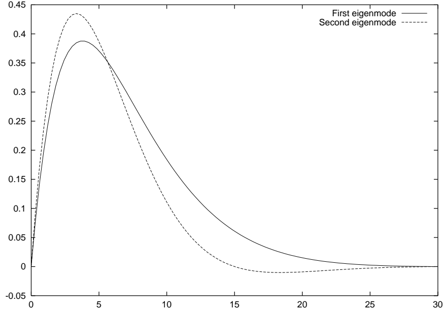
Figure 2: First two eigenmodes of the operator A , with \kappa = 4 and x^* = 30 years. Note the maxima situated at short maturities.
