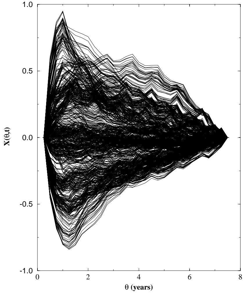
Figure 1: Various configurations adopted by the function X_t(x) defined in Eq. 5 as obtained from Eurodollar future contracts (1992-7). This figure may be seen as a visualization of the stationary density of the process X_t .
